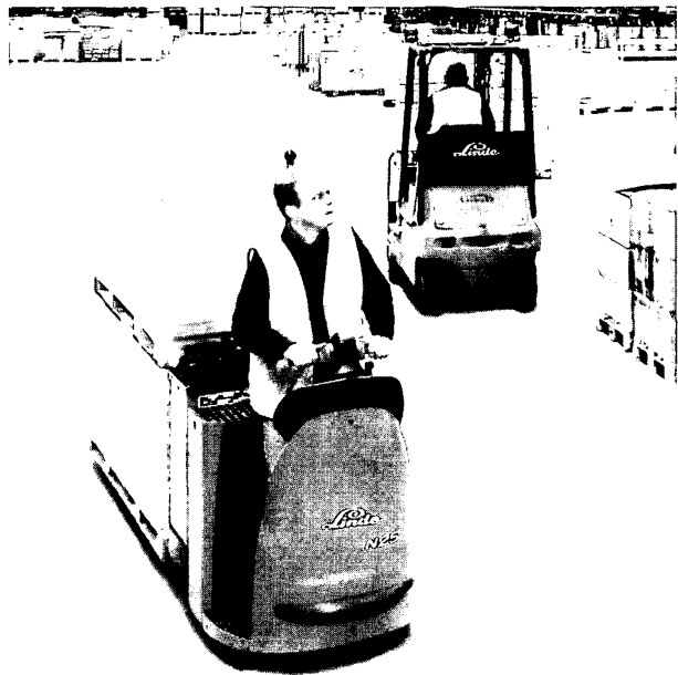
Figure 3.13: The small wheels on pallet trucks (such as that in the foreground) can be damaging to joints in floors.
