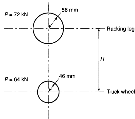
Figure B5: Equivalent loaded areas for racking legs and fork-lift truck wheels.
