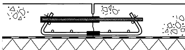
Figure 8.1: Sawn free-movement joint
