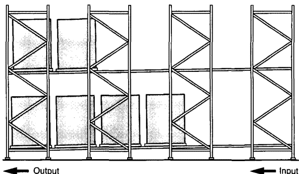
Figure 3.6: Live storage systems.
