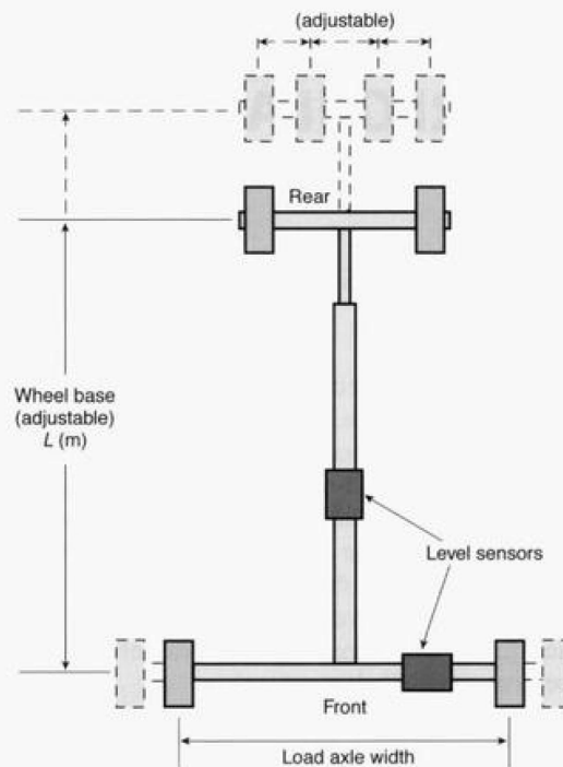
(b) Schematic of profilegraph
