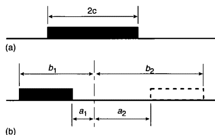
Figure 9.9: Defined areas of uniformly distributed load.
