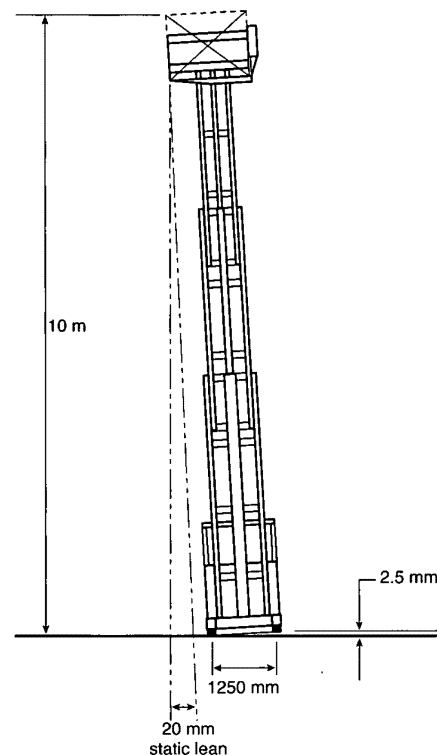
Figure 4.6: Static lean.
