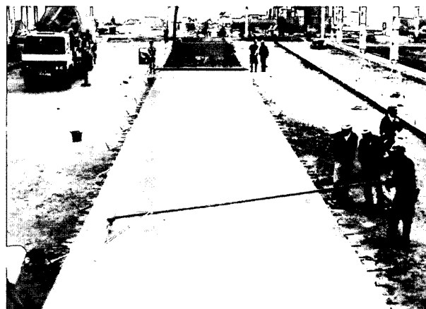
Figure 2.3: Long strip construction, allowing access for levelling using a highway straightedge.
